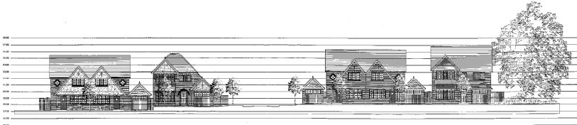
Street scene C-C
